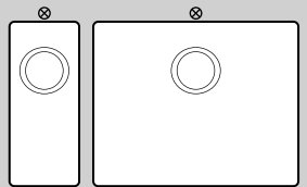
K1750 Bowl: 500 x 400 x 200 Slop sink: 170 x 400 x 170 Overall: 705 x 400 Partition: 35mm
