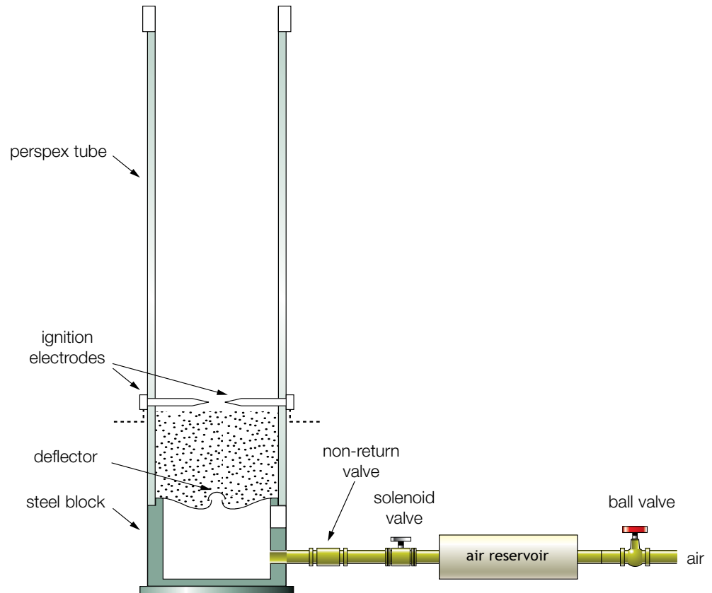
Figure 9 Vertical tube apparatus
