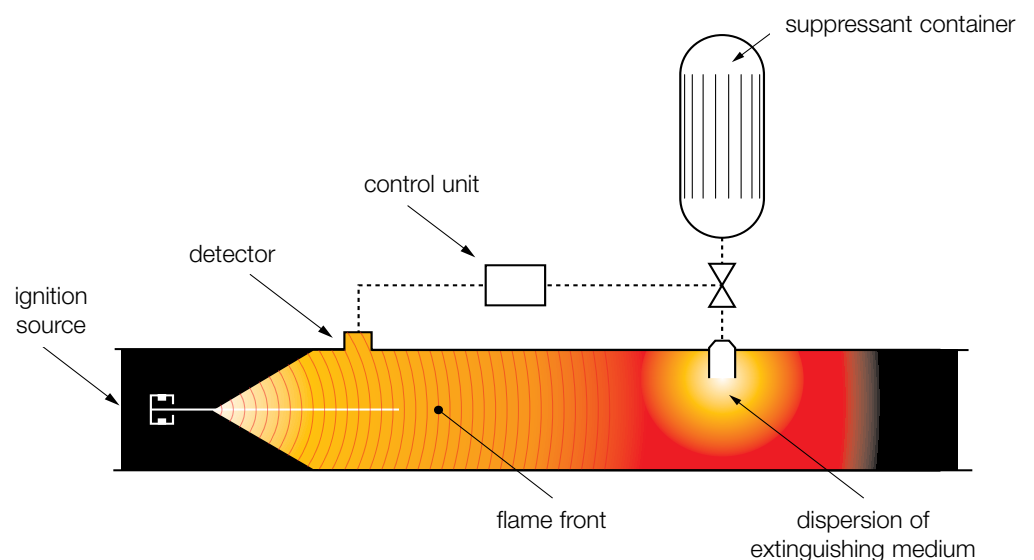
Figure 5 Suppressant barrier
