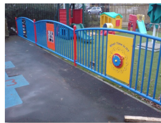
These railings are manufactured from 50mm round steel tubing with 25mm tubular vertical bars, they have coloured polyethylene infill panels. Available with a range of graphics and activities engraved on one side.
