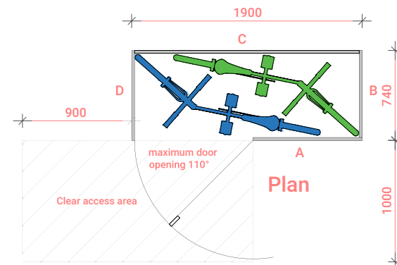
Warrior 2 Left Handed Horizontal Bike Locker
