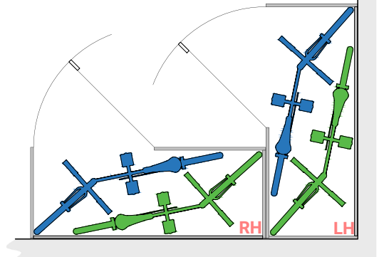
Warrior 2 Right Handed Horizontal Bike Locker
