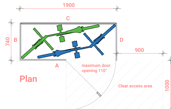
Warrior 2 Right Handed Horizontal Bike Locker
