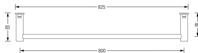
Installation with hat rosette R25H:
