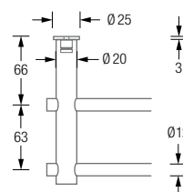
Product example HS20-140D800 Detail view:
