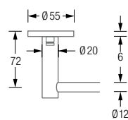
Product example HS20-80E800-K55 Detail view:
