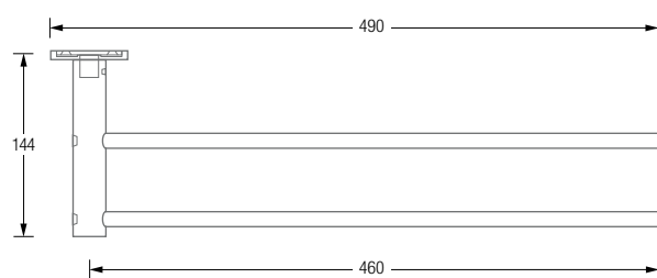
HS26-140EDS460 Plan view:
