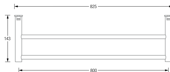
Product example HS20-140ED800 Plan view:
