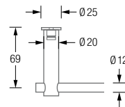
Product example HS20-80-800 Detail view:
