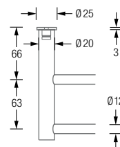
Product example HS20-140ED800 Detail view:
