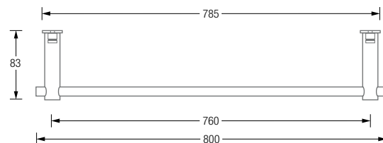
Product example HS20-80-800 Plan view:
