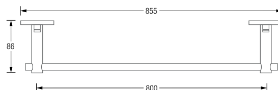
Product example HS20-80-800-K55 Plan view:
