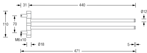
GHH2 Side view:
