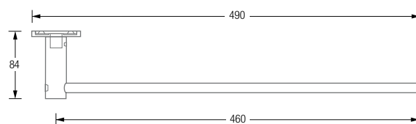
HS26-140EDS460 Plan view:
