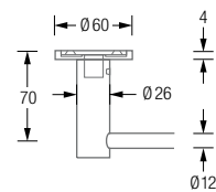
HS26-140EDS460 Detail view:
