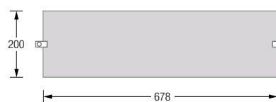
TOG-B Plan view:
