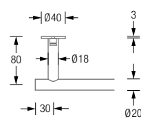
Product example HS18-800T Detail view:
