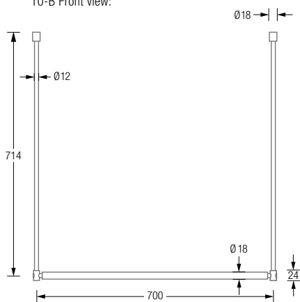
T0-B Front view:
