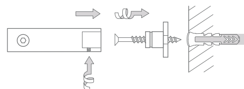
Installation with hat rosette R25H:
