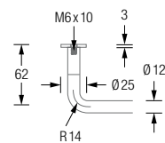
Product example HS12-800G Detail view:
