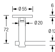
Product example HS20-80-800-K55 Detail view:
