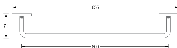
Product example HS12-800G-K55 Plan view:
