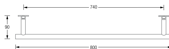
Product example HS18-800T Plan view:
