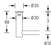
Product example HS20-80E800 Detail view:
