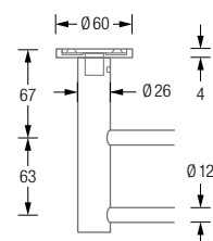
HS26-140EDS460 Detail view:
