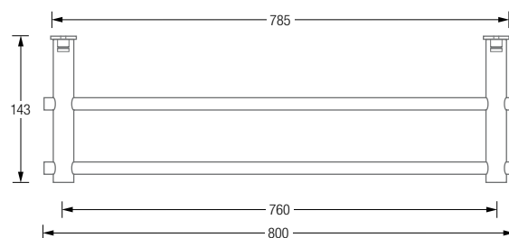
Product example HS20-140D800 Plan view:
