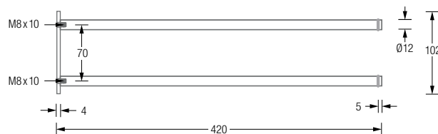
Product example HS12-420D-0 Plan view:
