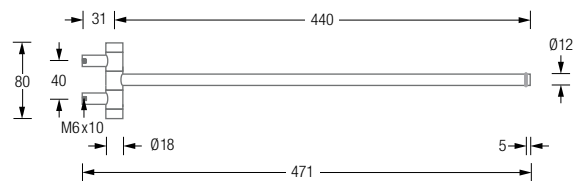
GHH2 Side view:
