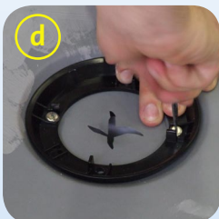
d. Secure the clamping ring with screws
