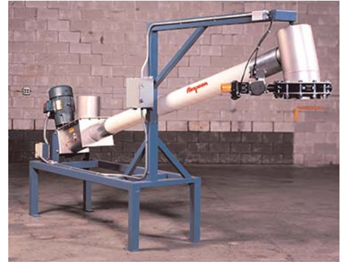
Motor drive at material inlet allows conveyor to fit in low headroom areas.
