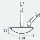
SGL Pilaster Section
