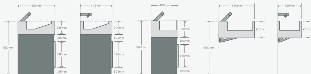
Hydra Solid Surface Washtroughs with deck mounted taps and underframe
