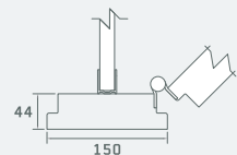
HPL/Veneer Pilaster Section
