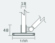
MFC/HPL/Real Wood Veneer Pilaster Section
