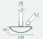
MFC/HPL/Real Wood Veneer Pilaster Section
