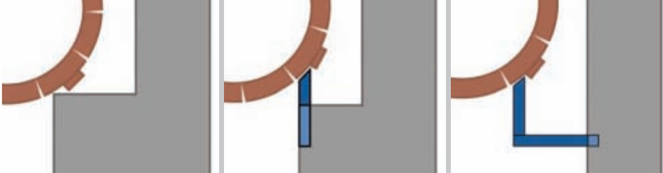
Standard reveal 400 mm + No fascia needed Inward fascia Angled corner fascia 120 mm
