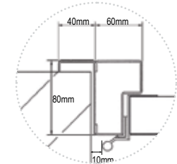
Frame dimensions
