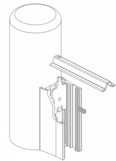
Top (during installation) Gova clip
