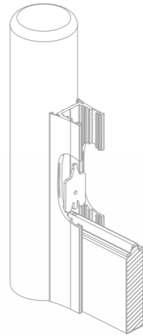
Top (during installation) gova clip + gova-set-screw
