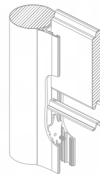
Bottom (during installation) gova clip + gova-set-screw
