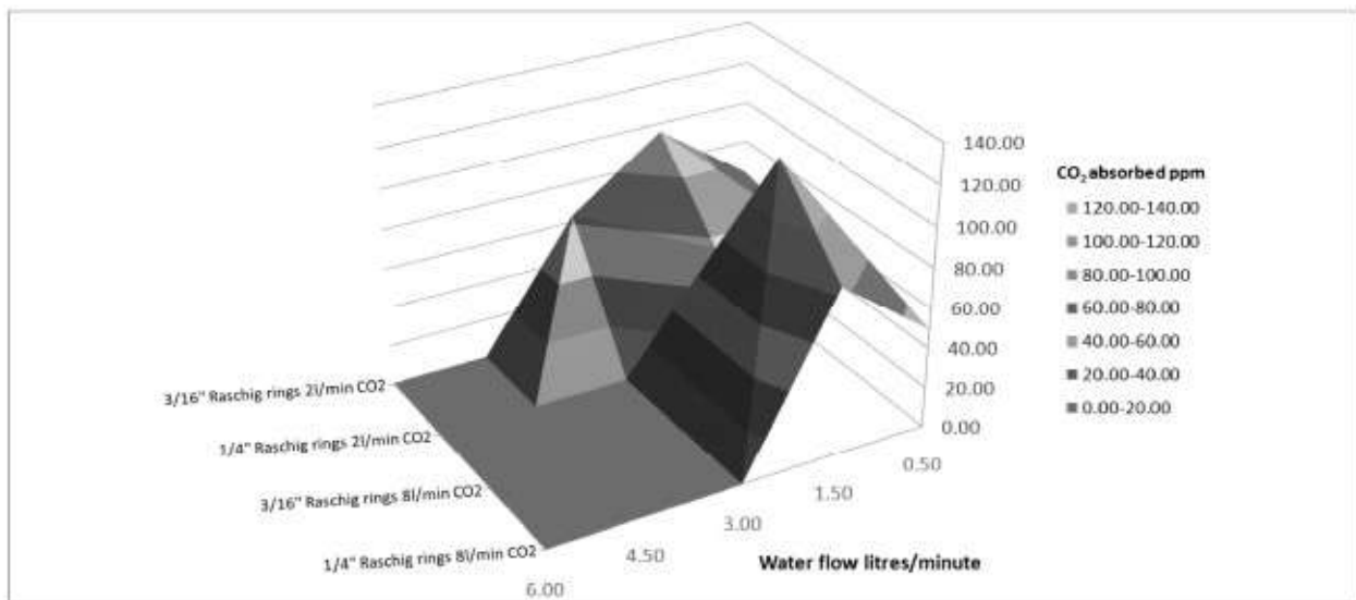
Figure 5: Graph of Raschig ring performance.
