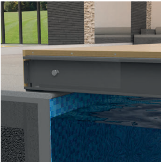
Pool-span beams with a padded underside to protect the edge of the pool.
