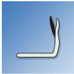
Angle Jamb Glass to Wall Shower Seal
