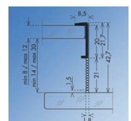
Glass Lip Seal Kit detail
