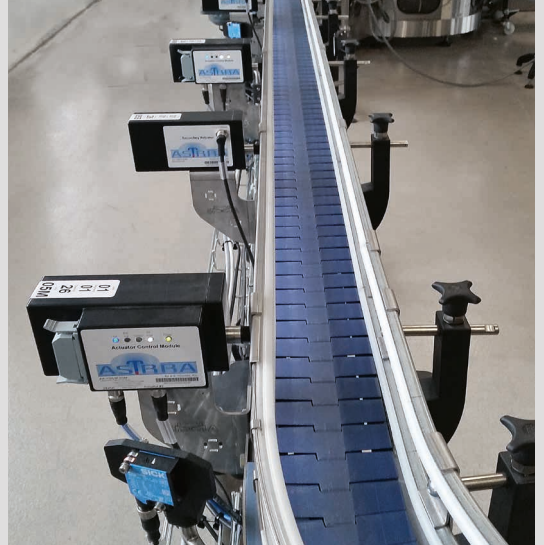
Automatically adjustable side rails ASTRA
