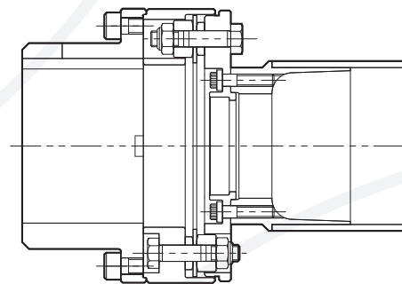
Optional Bolted Cartridge Assembly
