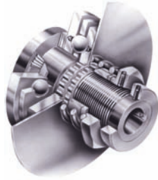
Autogard Series 200 Torque Limiters
