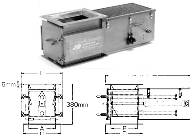
Dimensions and Openings for Pneumatic Self-Cleaning Models (in mm)
