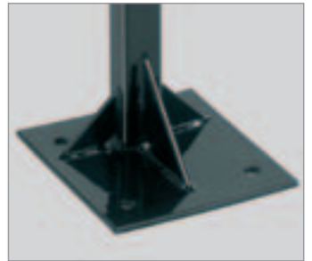
bolt down post and colour coating
