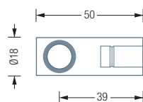
HG18-50D Side view:
