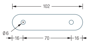
ROV23-B6 Top view:
