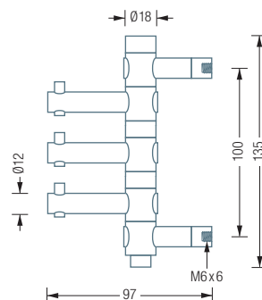
GH3 Side view:
