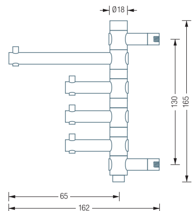
GH4-2 Side view:
