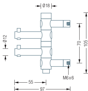
GH2 Side view:
