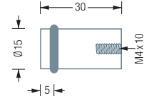
HG15-30 Side view:
