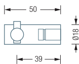
H18-50D Side view:
