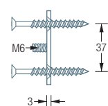
R55S Side view:
