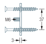
R55VN Side view:
