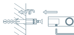
HG18-50D Wall mounting:
