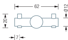
H18-50D Front view:
