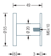
HA3-R55S55 Side view:
