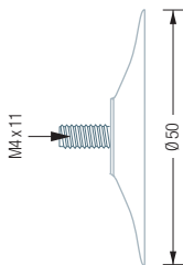
SN50-11 Side view:
