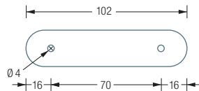
ROV23-B4 Top view:
