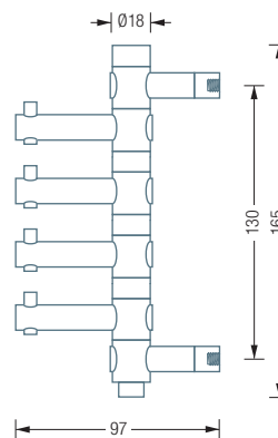
GH4 Side view:
