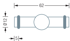
HG18-50D Front view:
