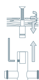
HG18-50D Cabinet base assembly:
