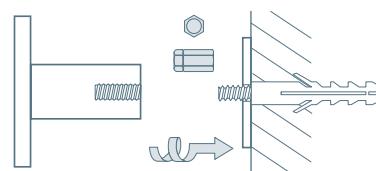
Wall mounting with rosette:
