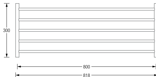
Product example SR800-2 / -3 Plan View:
