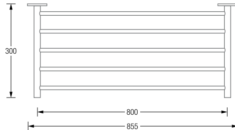
Product example SR800-1W Plan View:
