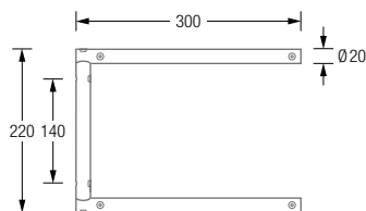
Product example SR800-2W Side View:
