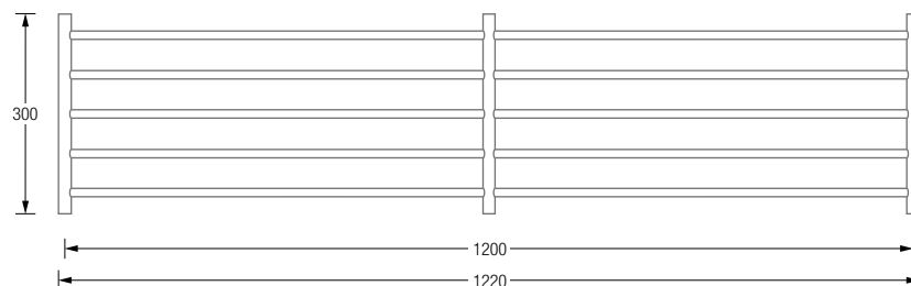
Product example SR1200-4 / -5 Plan View:
