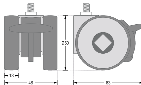
Floor castor with brake:
