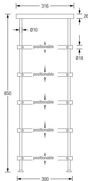
Product example SBS800-5-Oak Side View:
