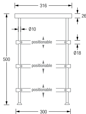
Product example SB800-3-Oak Side View:
