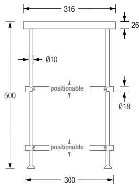
Product example SB1200-2-Oak Side View:
