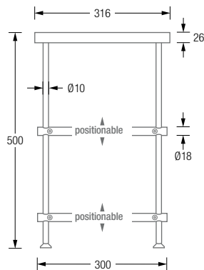
Product example SB800-2-Oak Side View:
