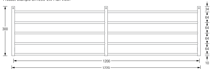
Product example SR1200-2W Plan View:
