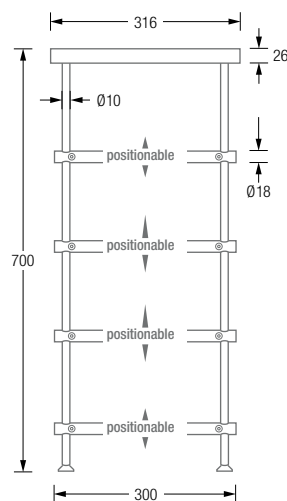
Product example SBS800-4-Oak Side View:
