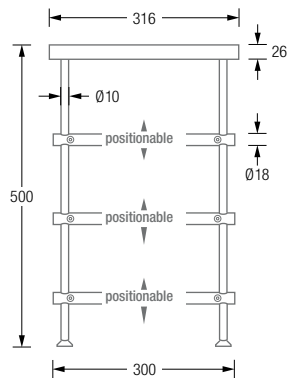
Product example SB1200-3-Oak Side View:
