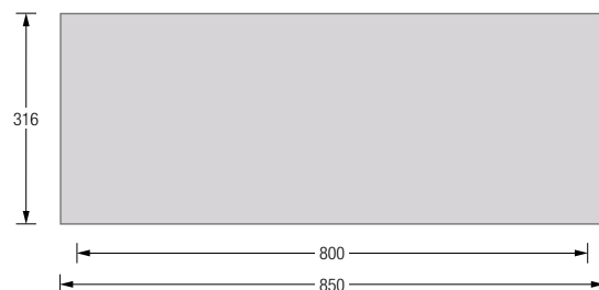
Product example SBS800-4-Oak / -5-Oak Plan View:
