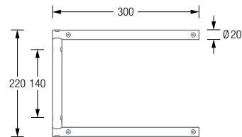
Product example SR1200-2W Plan View:
