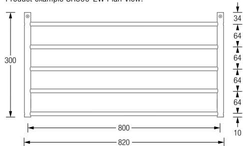
Product example SR800-2W Plan View:
