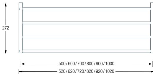
G18-500 / 600 / 700 / 800 / 900 / 1000 Plan View:
