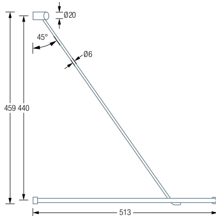
G500VW Side View:
