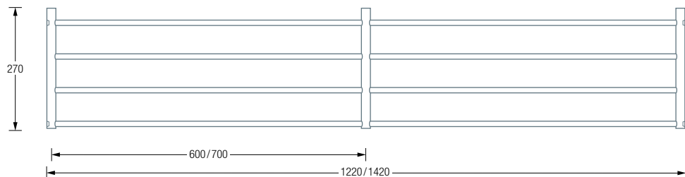
G15-1200 / 1400 Plan View:
