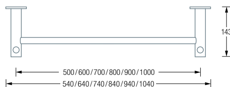
G4-500 / 600 / 700 / 800 / 900 / 1000 Plan View:
