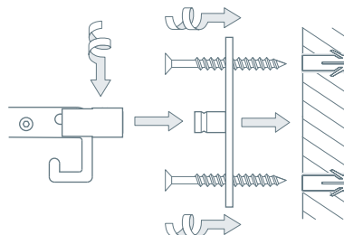
Installation with oval rosette:
