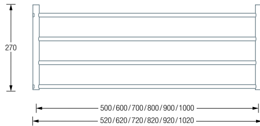
G15-500 / 600 / 700 / 800 / 900 / 1000 Plan View:
