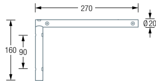
G15 Side View:
