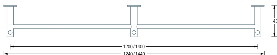
G4-1200 / 1400 Plan View:
