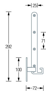
KLR600 / 700 / 800 / 900 Side View Folded:
