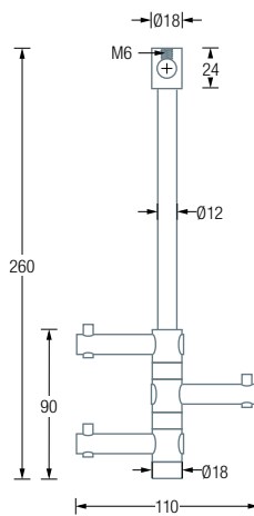
T3F Side View:
