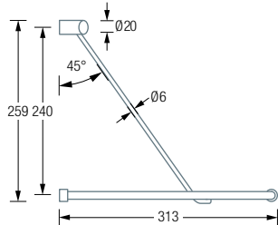
G300VW Side View:
