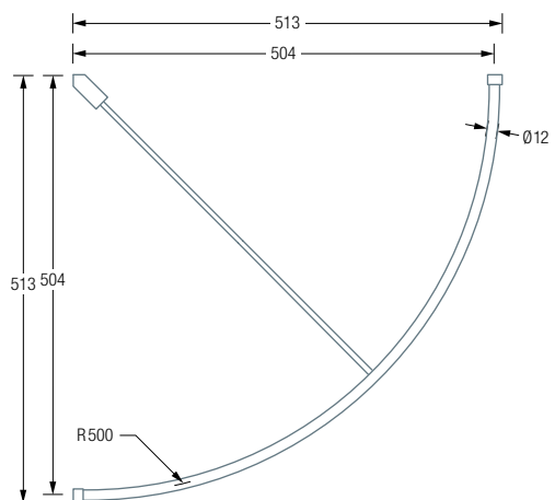
G500VW Plan View:
