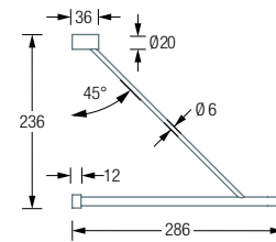
GU1 Side View:
