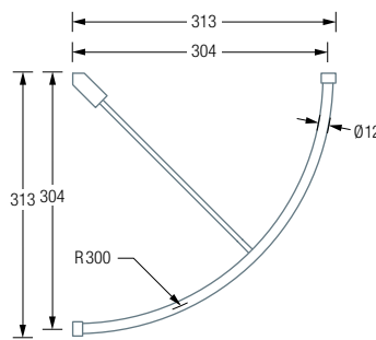
G500VW Plan View:
