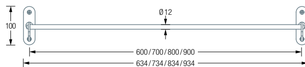
KLR600 / 700 / 800 / 900 Front View Folded:
