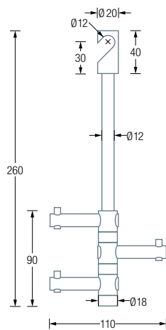
T3H Side View:
