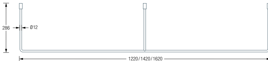
GU1-1200 / 1400 / 1600 Plan View:
