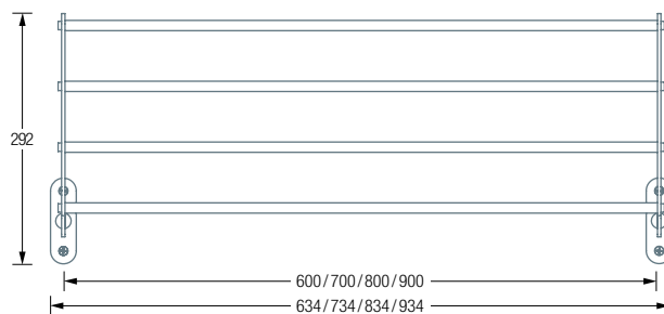
Installation with oval rosette:
