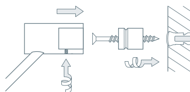
Mounting with mounting sleeve and wall bracket STF:
